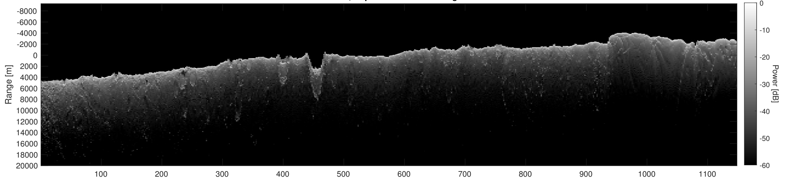
Orbit 13140, Depth-Corrected Cluttergram
