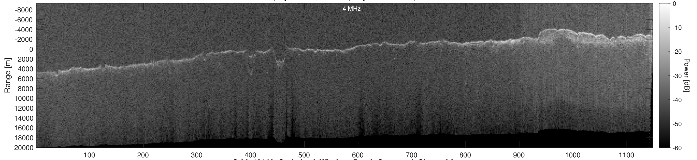
Orbit 13140, Optimized, Window, Depth-Corrected, Channel 2
