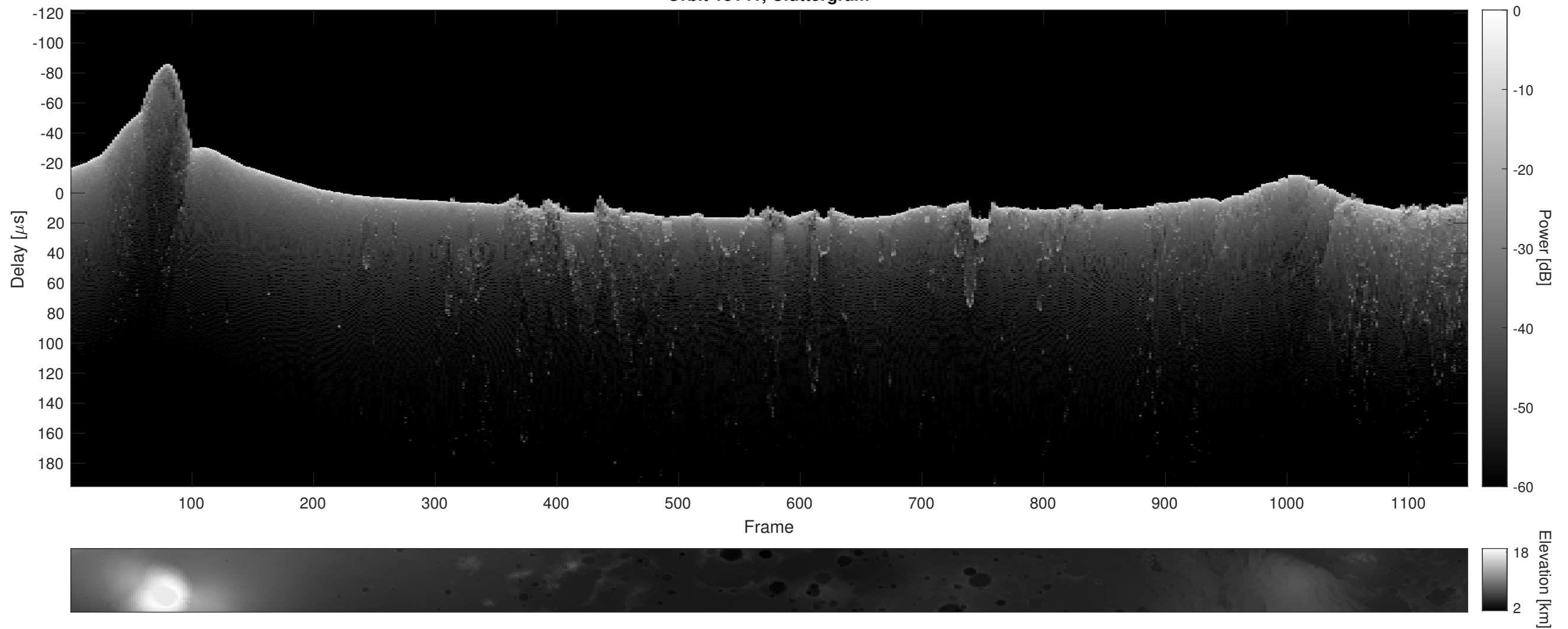
Orbit 13141, Cluttergram
