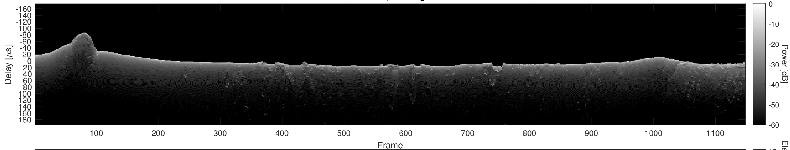
Orbit 13141, Cluttergram
