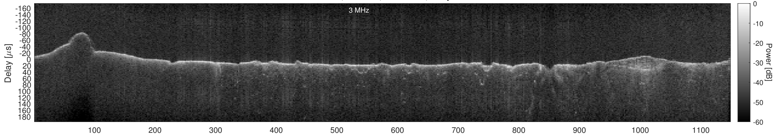
Orbit 13141, Window, Channel 2, Optimized
