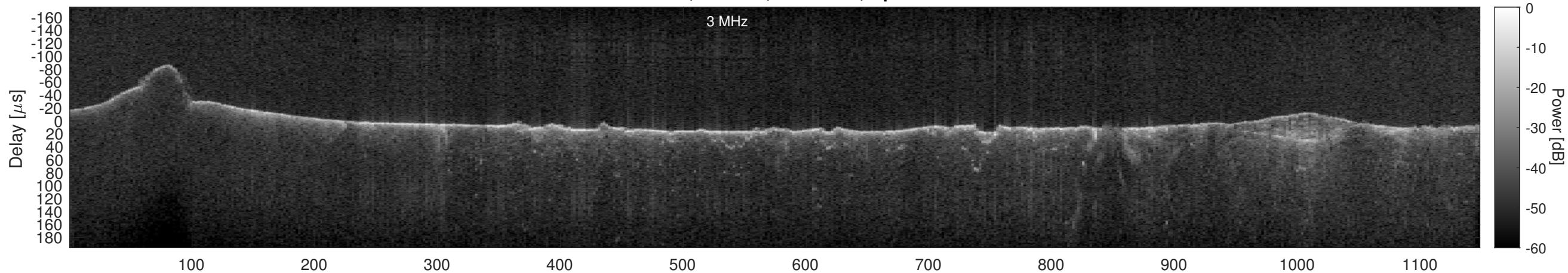
Orbit 13141, Cluttergram
