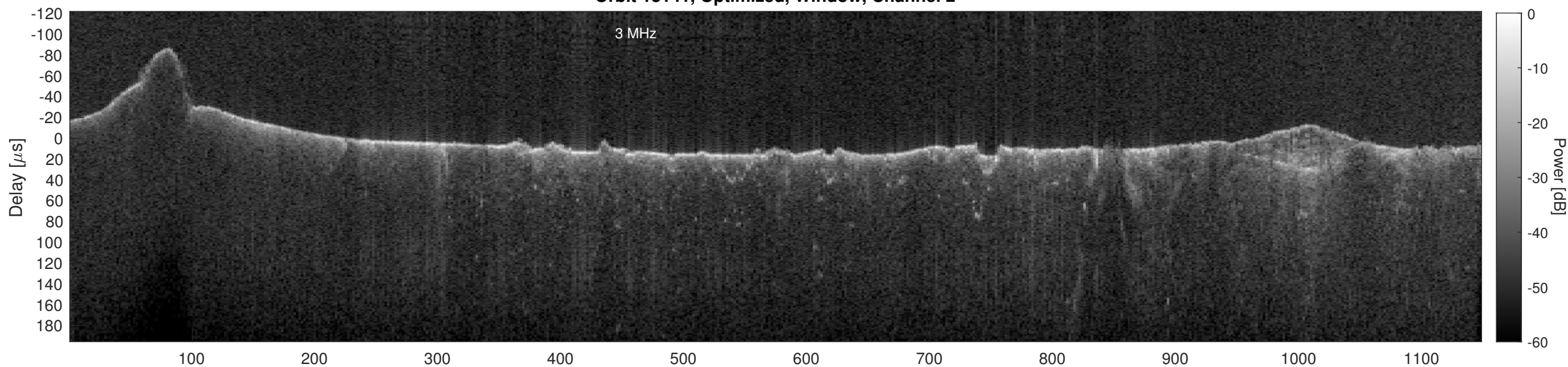
Orbit 13141, Cluttergram
