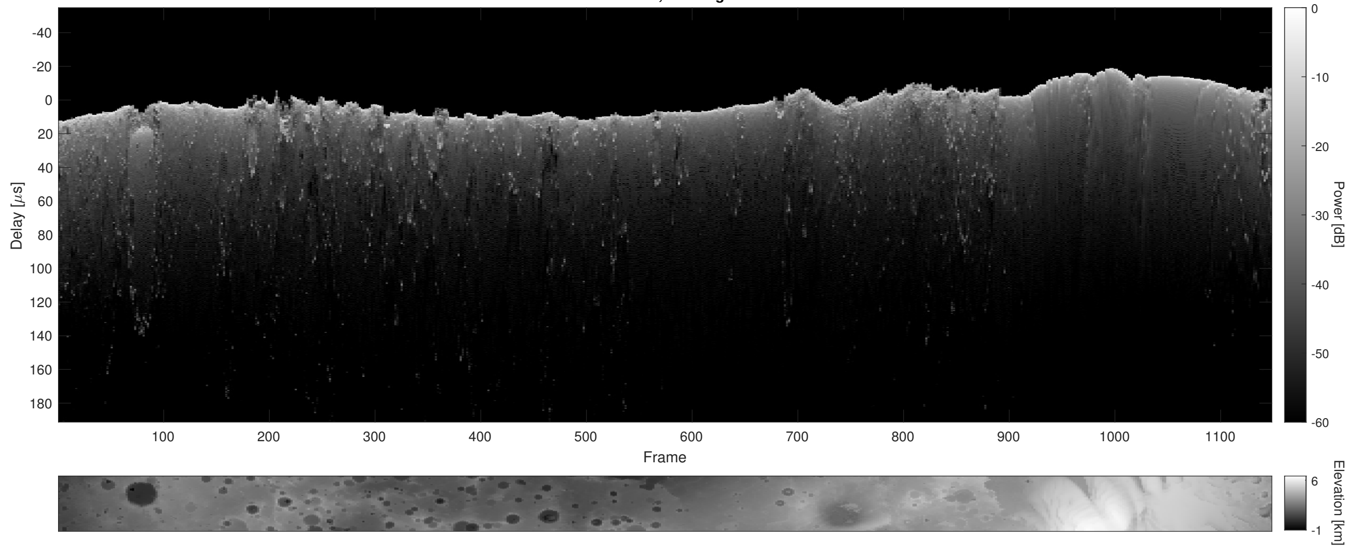
Orbit 13143, Cluttergram
