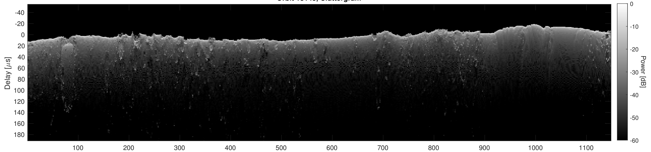
Orbit 13143, Cluttergram
