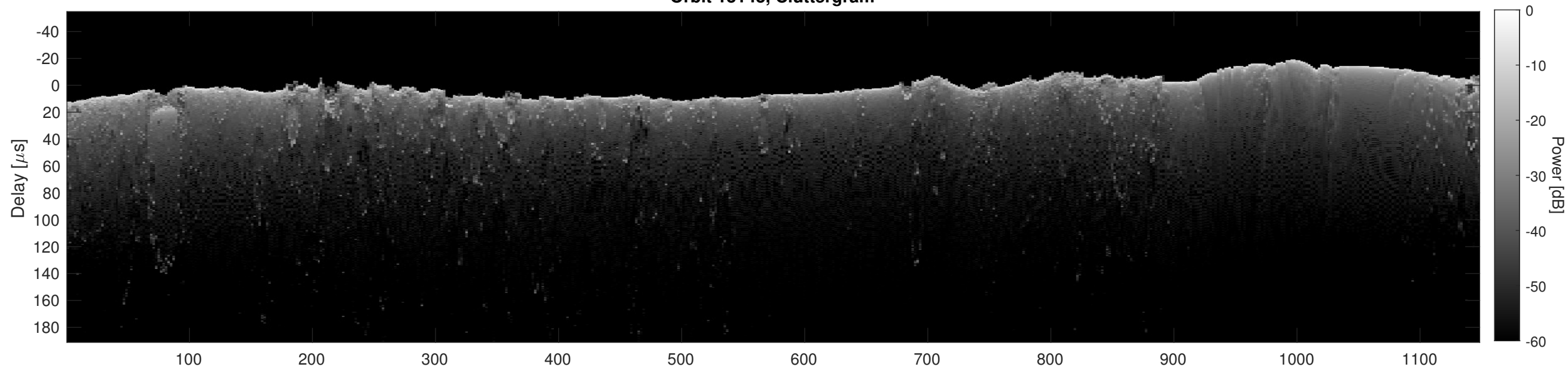
Orbit 13143, Cluttergram
