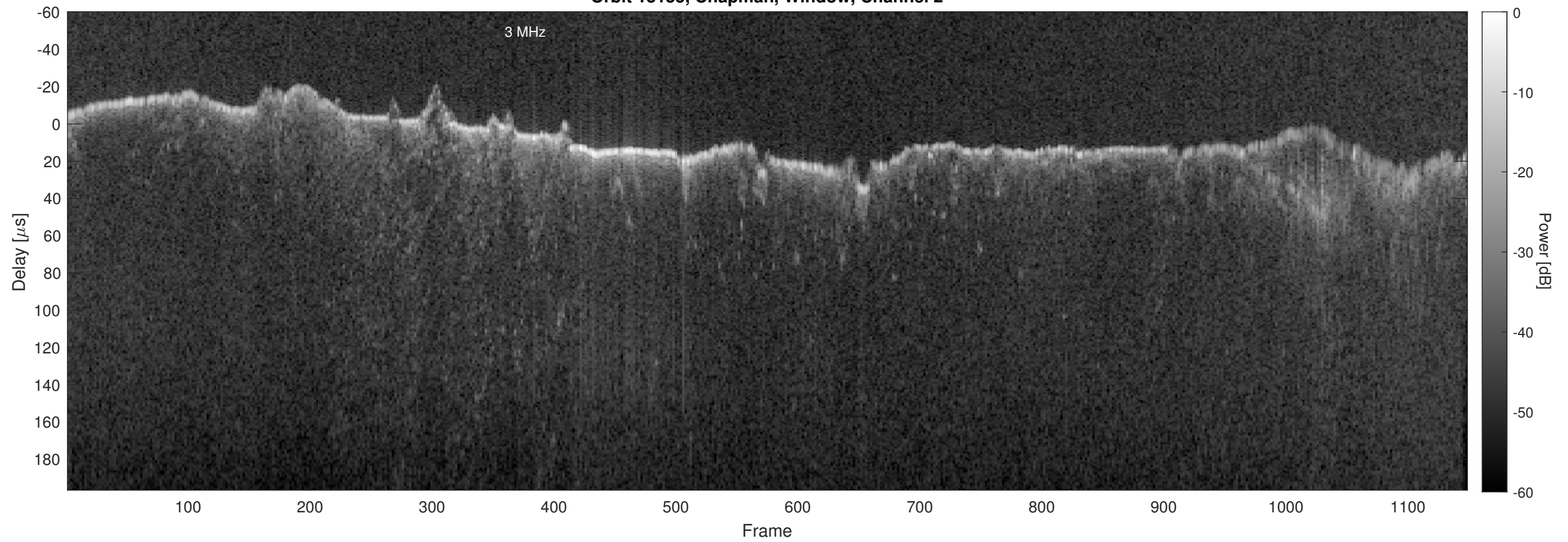
Orbit 13155, Chapman, Window, Channel 2
