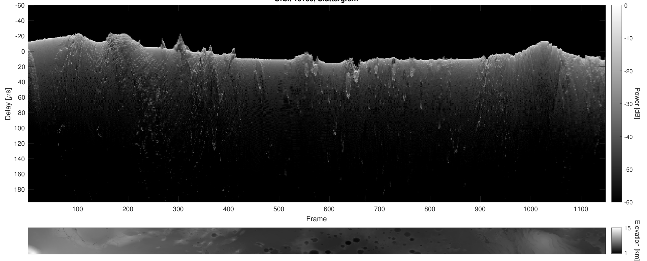
Orbit 13155, Cluttergram
