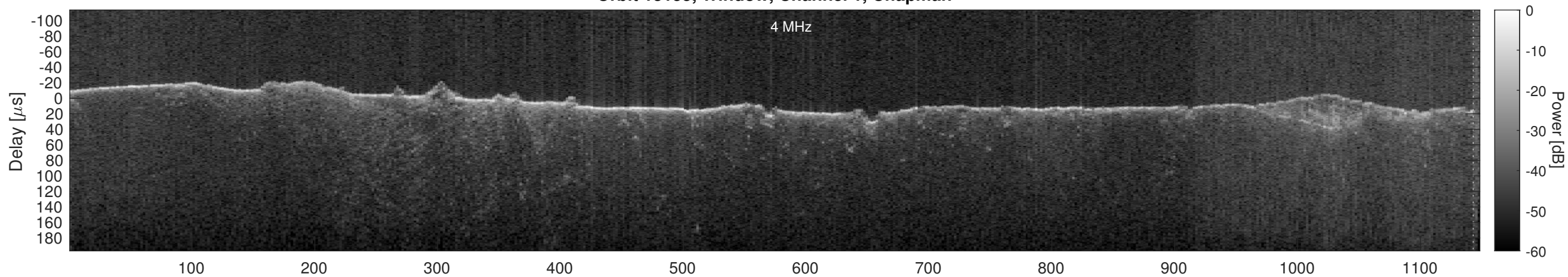
Orbit 13155, Window, Channel 1, Optimized
