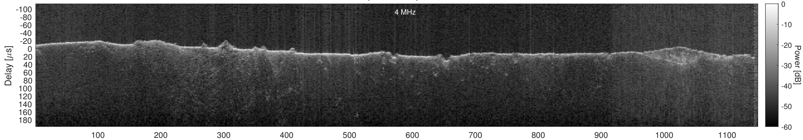
Orbit 13155, Window, Channel 1, Chapman
