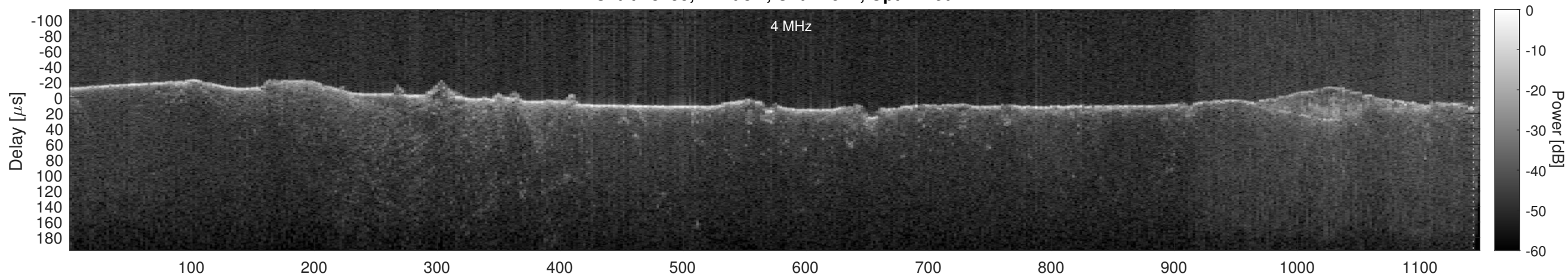
Orbit 13155, Cluttergram
