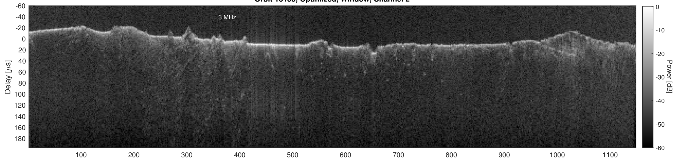
Orbit 13155, Cluttergram
