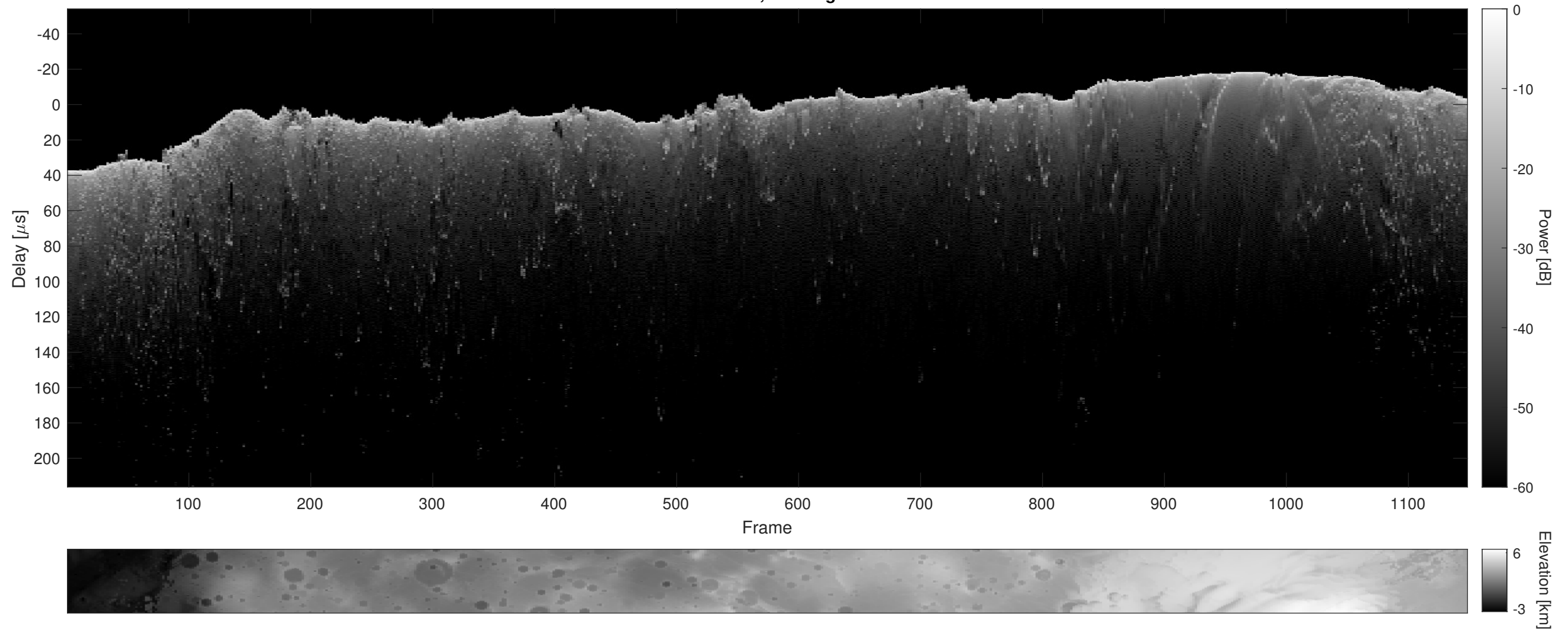
Orbit 13156, Cluttergram
