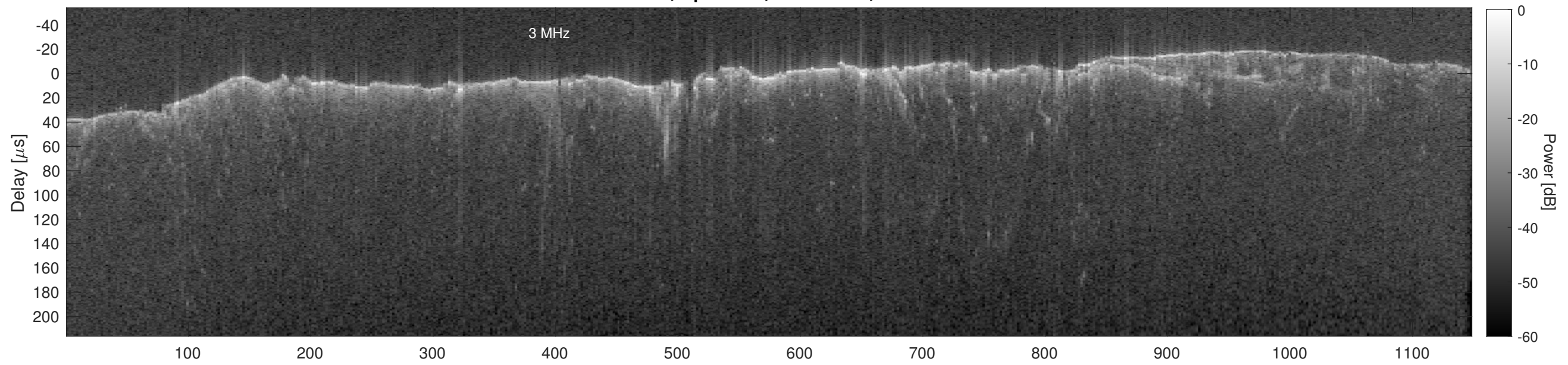
Orbit 13156, Cluttergram
