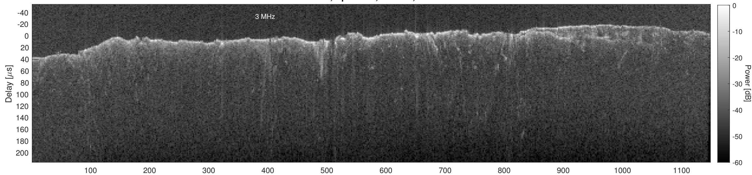
Orbit 13156, Cluttergram
