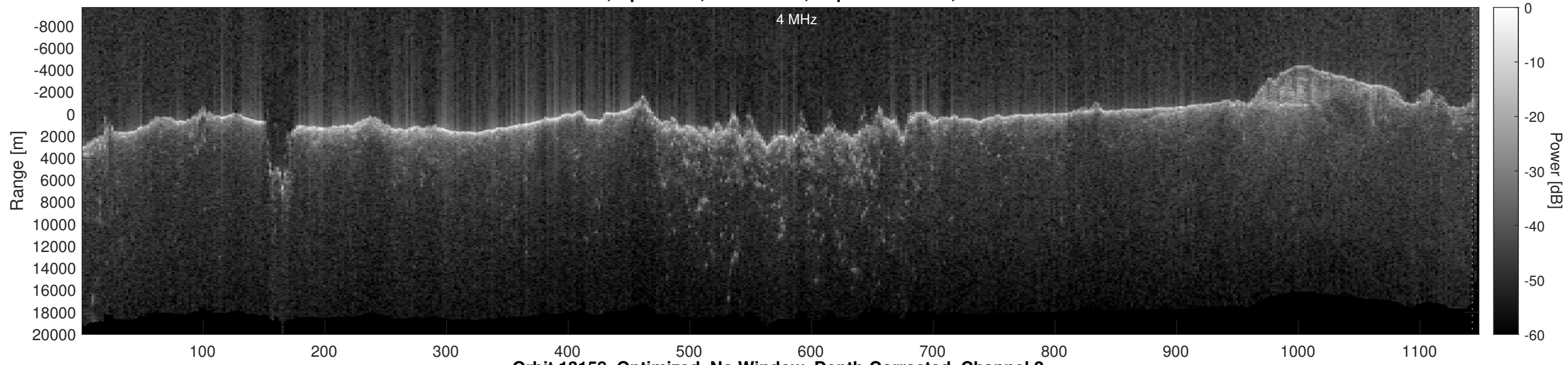
Orbit 13158, Optimized, No Window, Depth-Corrected, Channel 2
