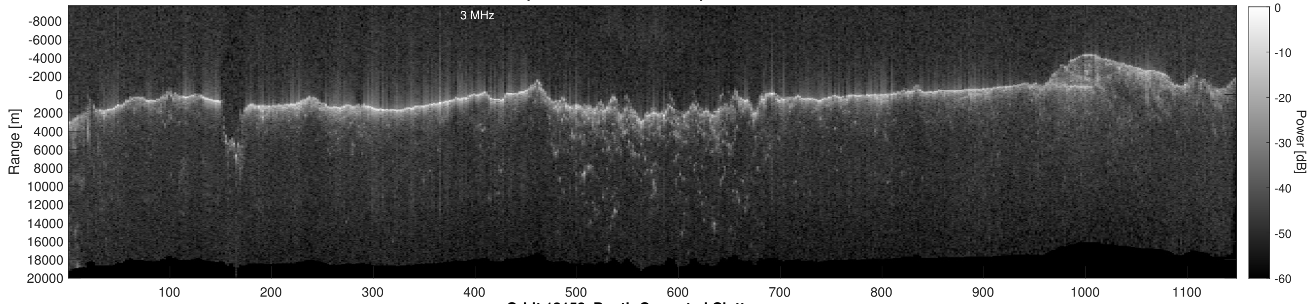
Orbit 13158, Depth-Corrected Cluttergram
