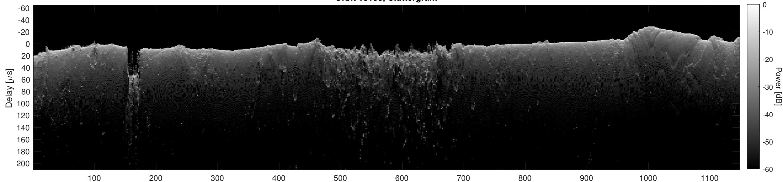
Orbit 13158, Cluttergram
