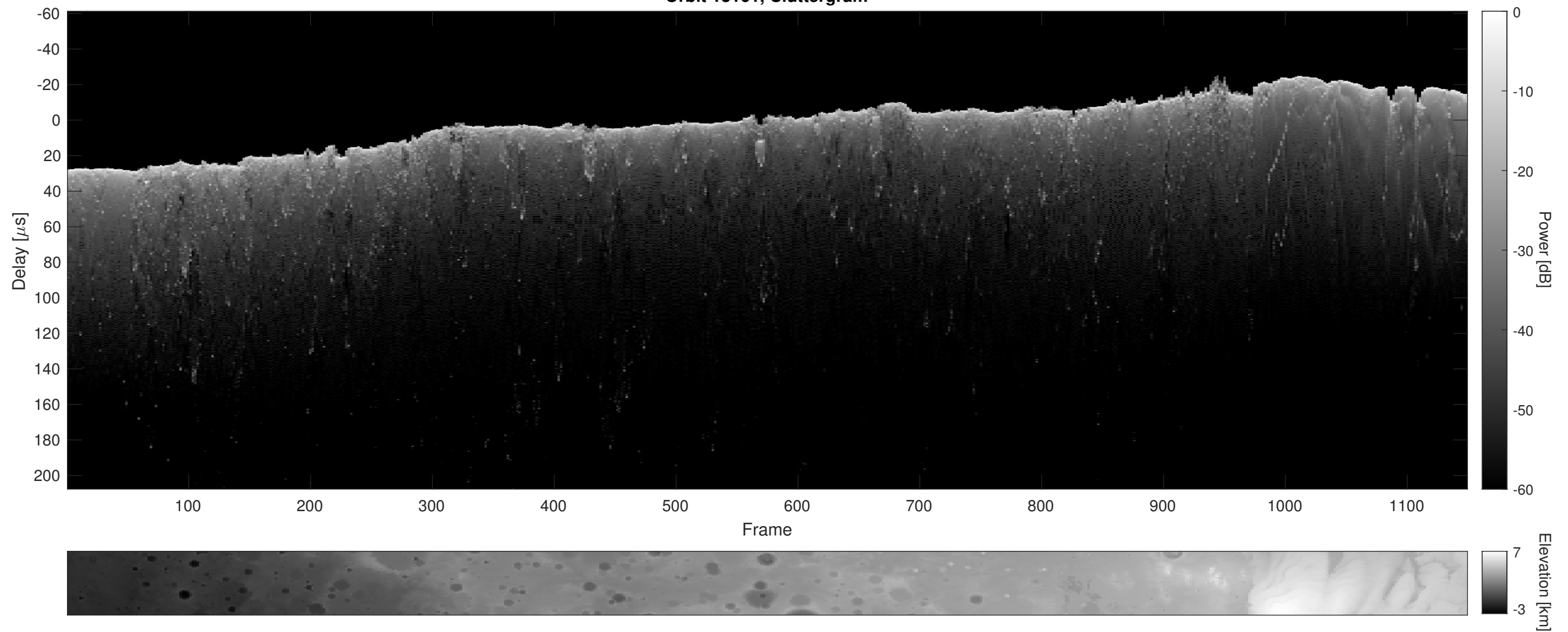
Orbit 13161, Cluttergram
