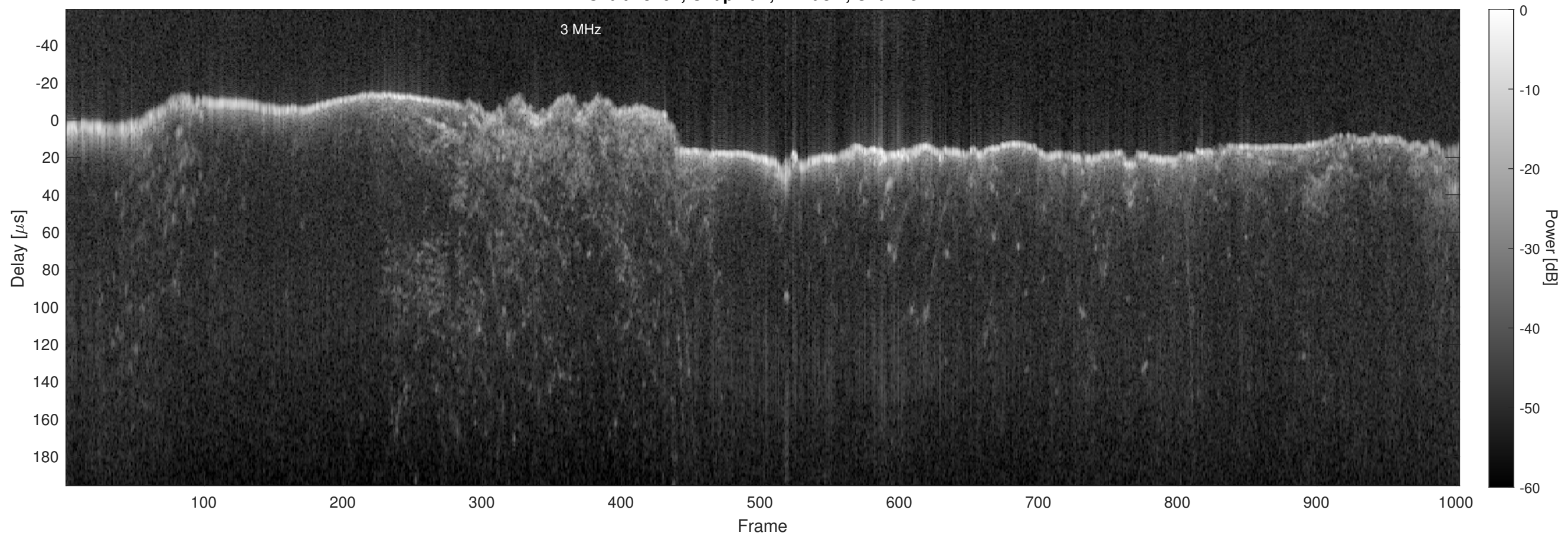
Orbit 13162, Chapman, Window, Channel 2
