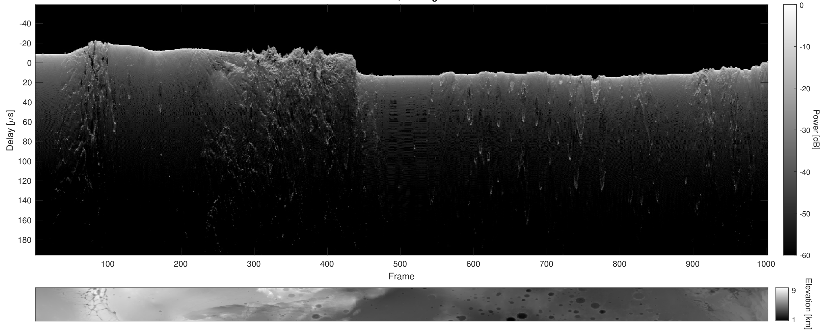
Orbit 13162, Cluttergram
