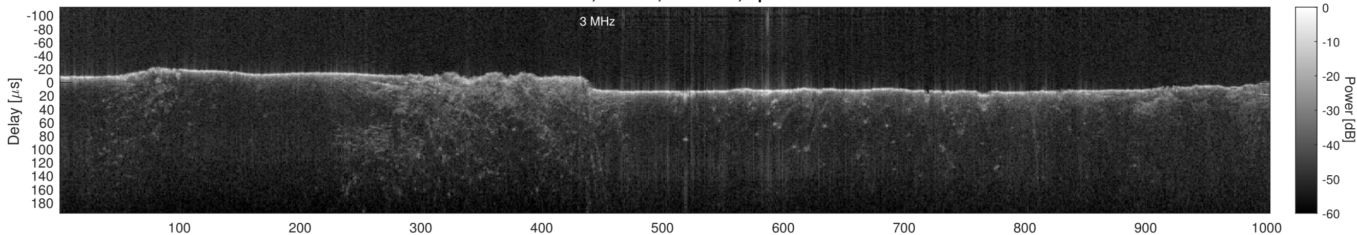
Orbit 13162, Cluttergram
