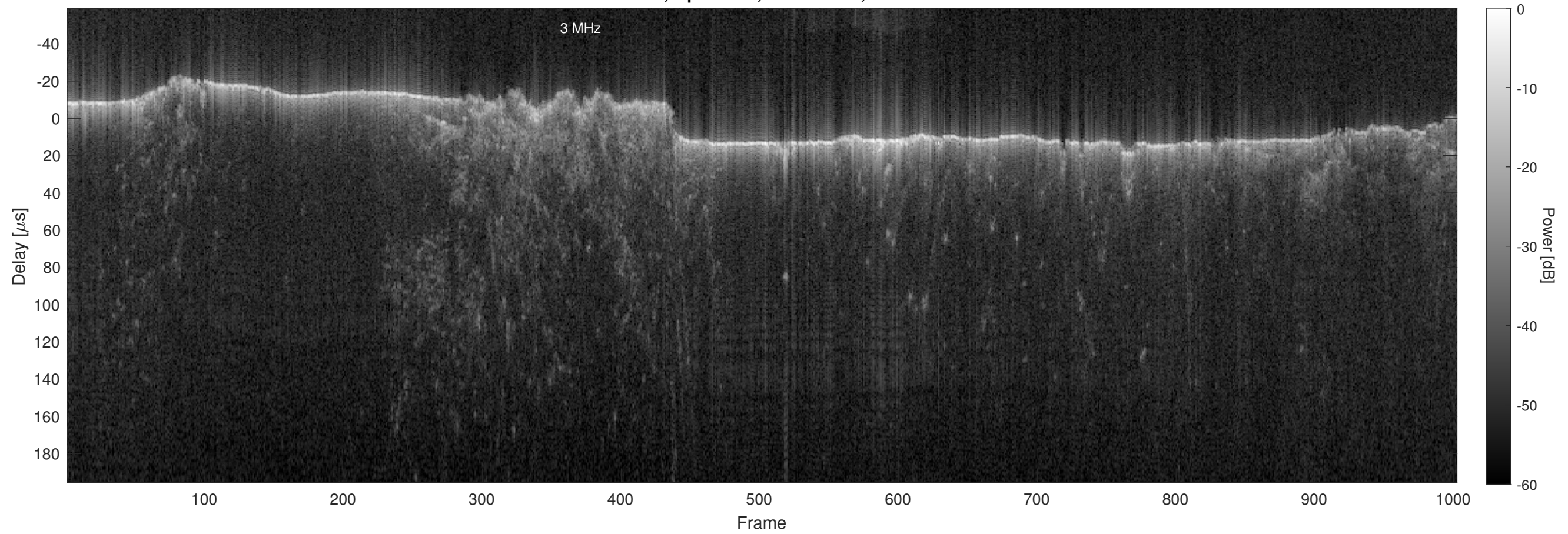
Orbit 13162, Optimized, No Window, Channel 2
