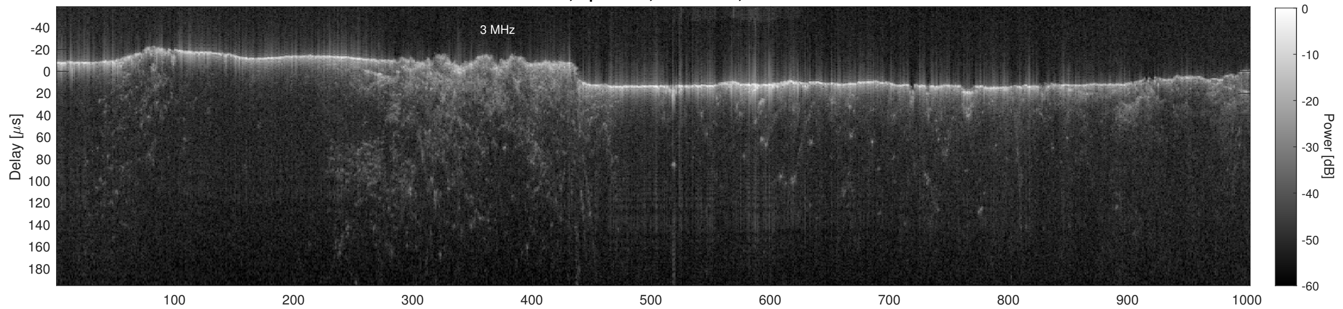
Orbit 13162, Cluttergram
