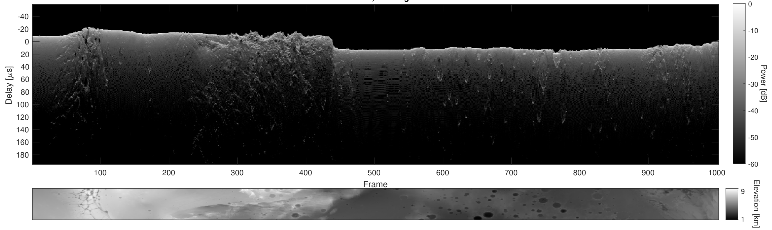
Orbit 13162, Cluttergram
