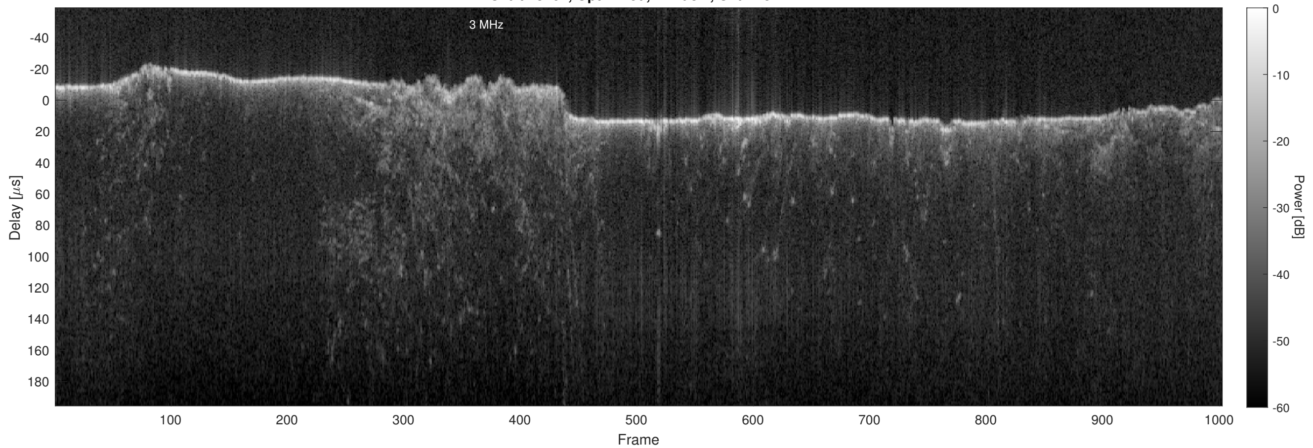
Orbit 13162, Optimized, Window, Channel 2
