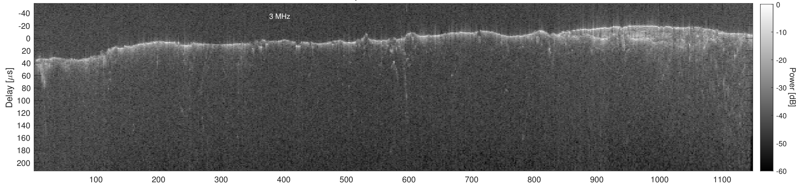
Orbit 13163, Cluttergram
