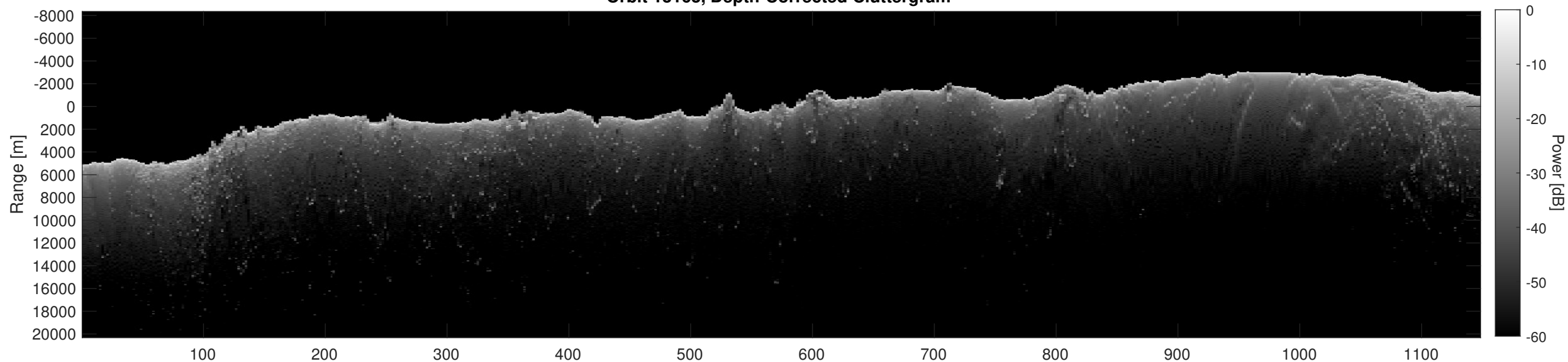
Orbit 13163, Depth-Corrected Cluttergram
