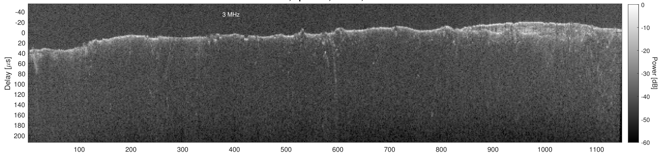
Orbit 13163, Cluttergram
