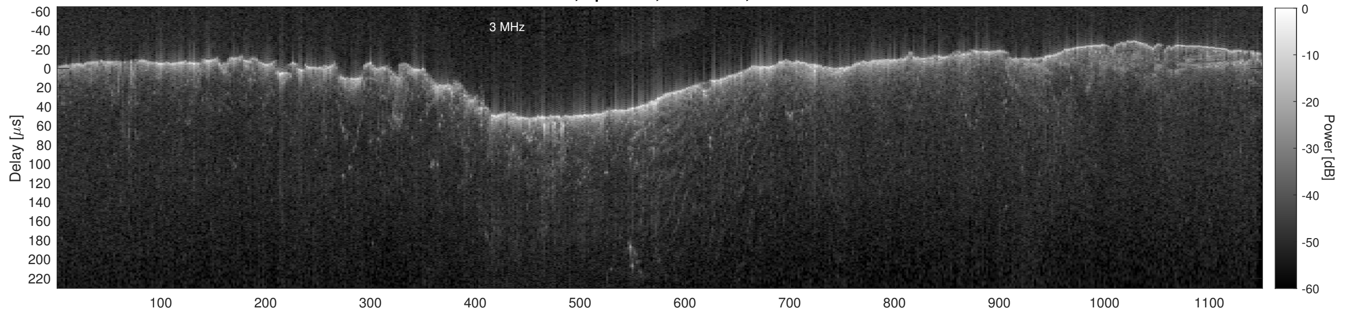
Orbit 13164, Cluttergram
