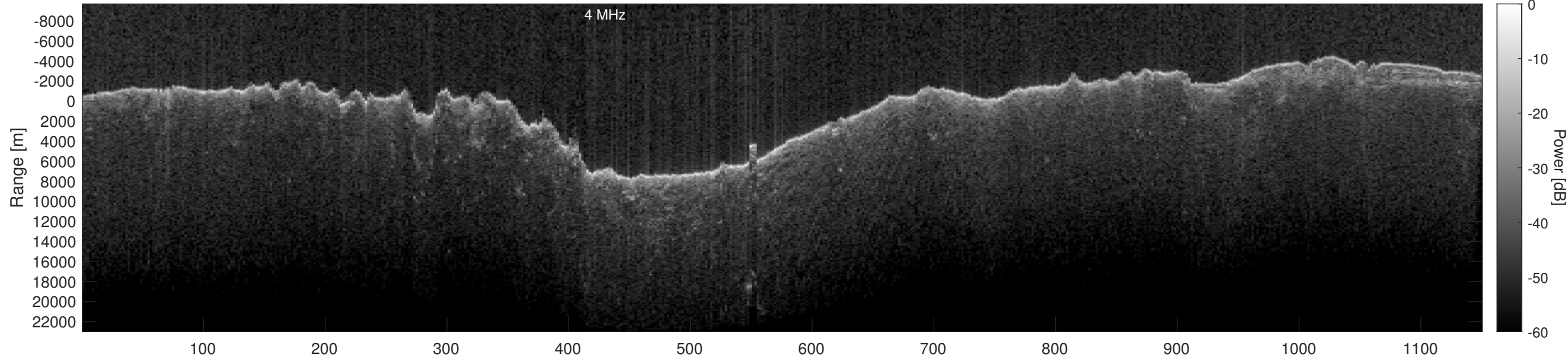
Orbit 13164, Optimized, Window, Depth-Corrected, Channel 2
