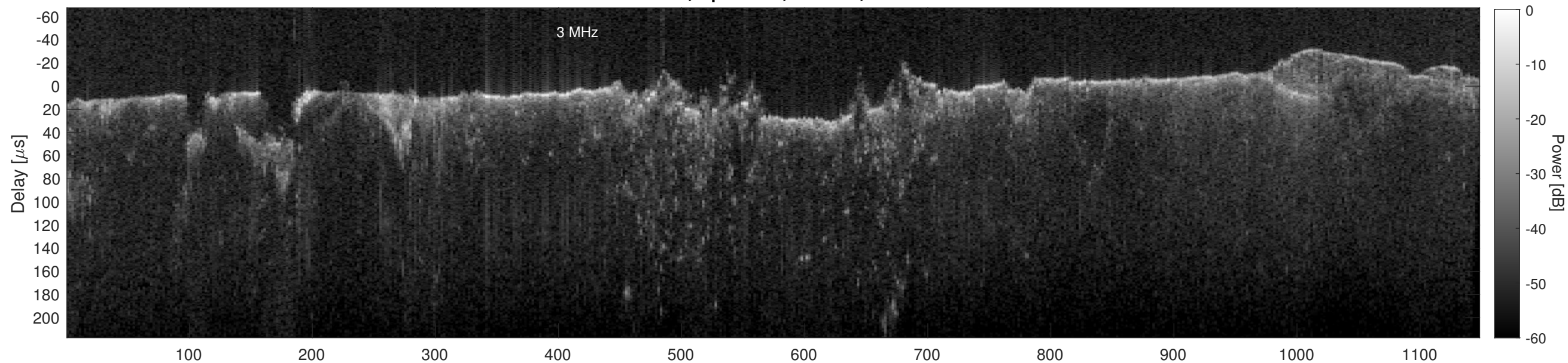
Orbit 13165, Cluttergram
