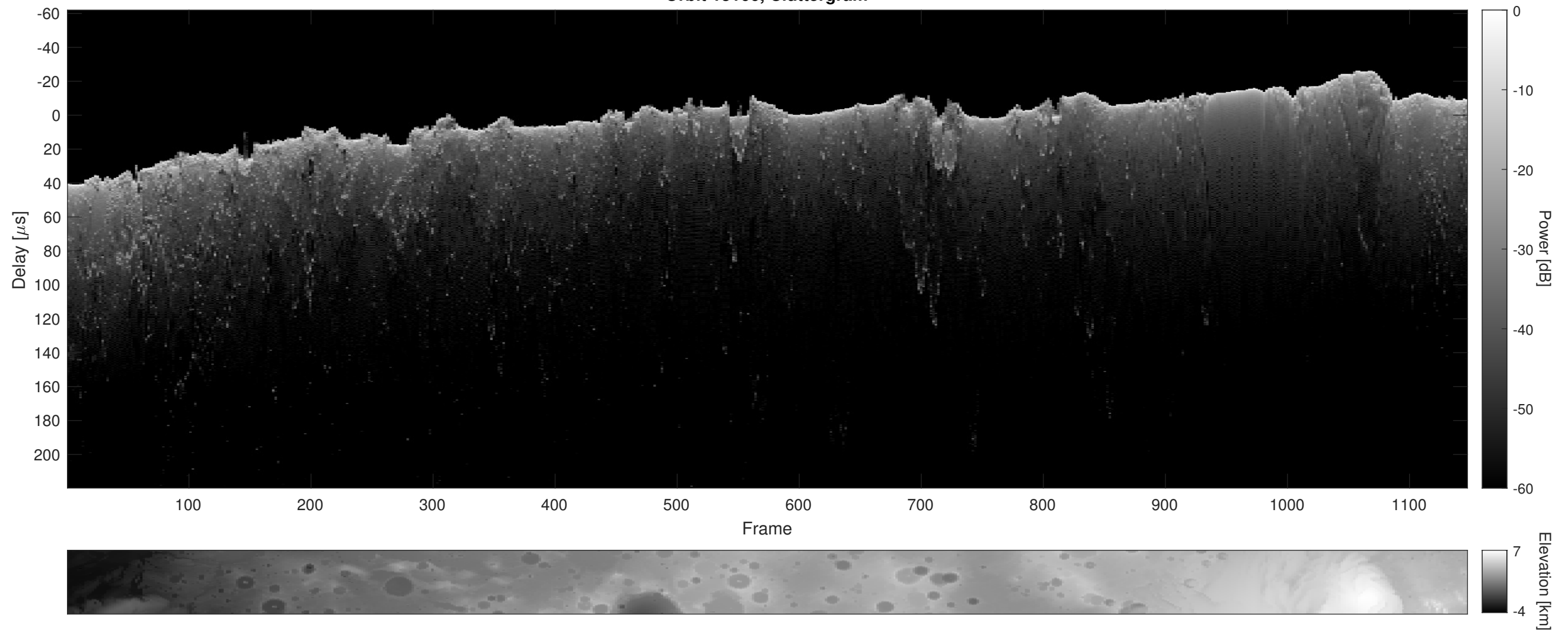
Orbit 13166, Cluttergram
