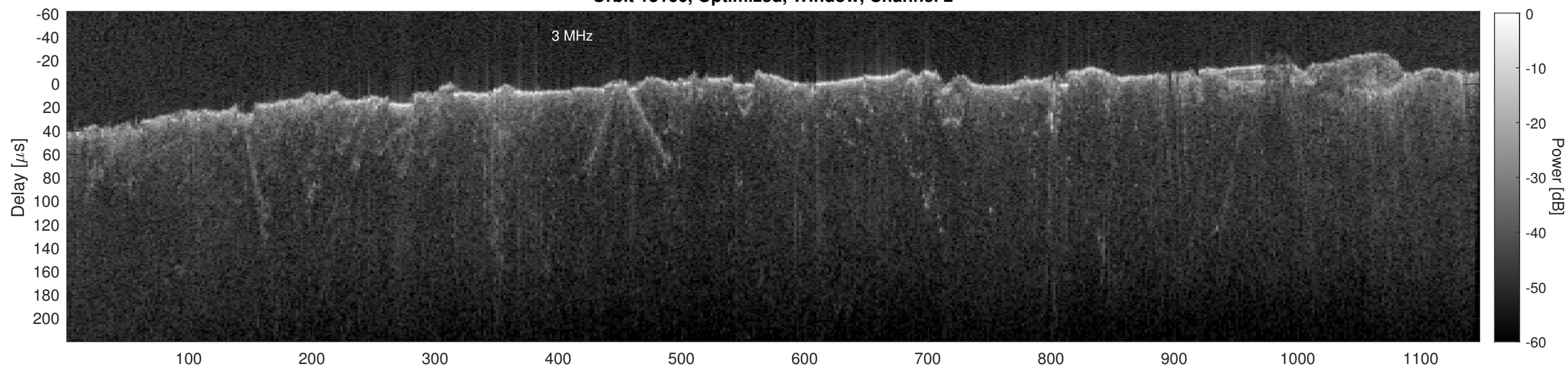
Orbit 13166, Cluttergram
