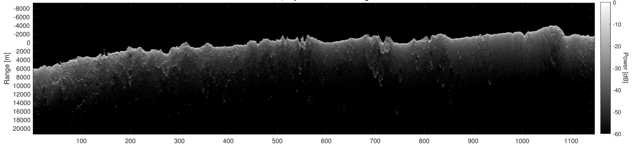
Orbit 13166, Depth-Corrected Cluttergram
