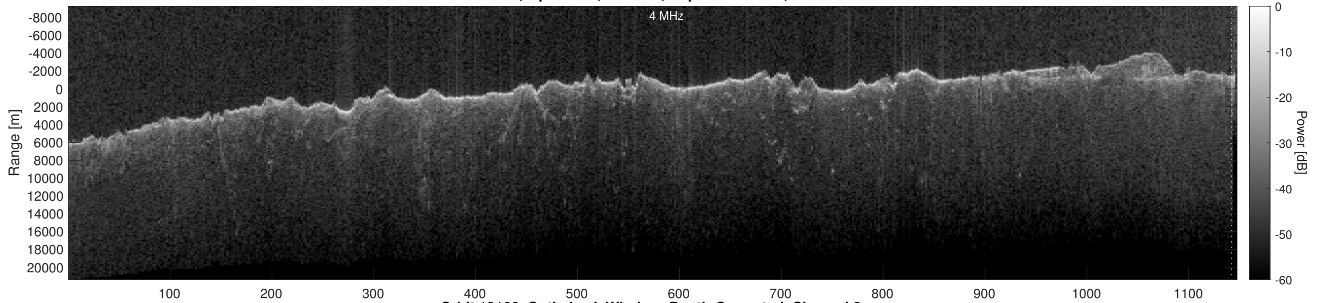
Orbit 13166, Optimized, Window, Depth-Corrected, Channel 2
