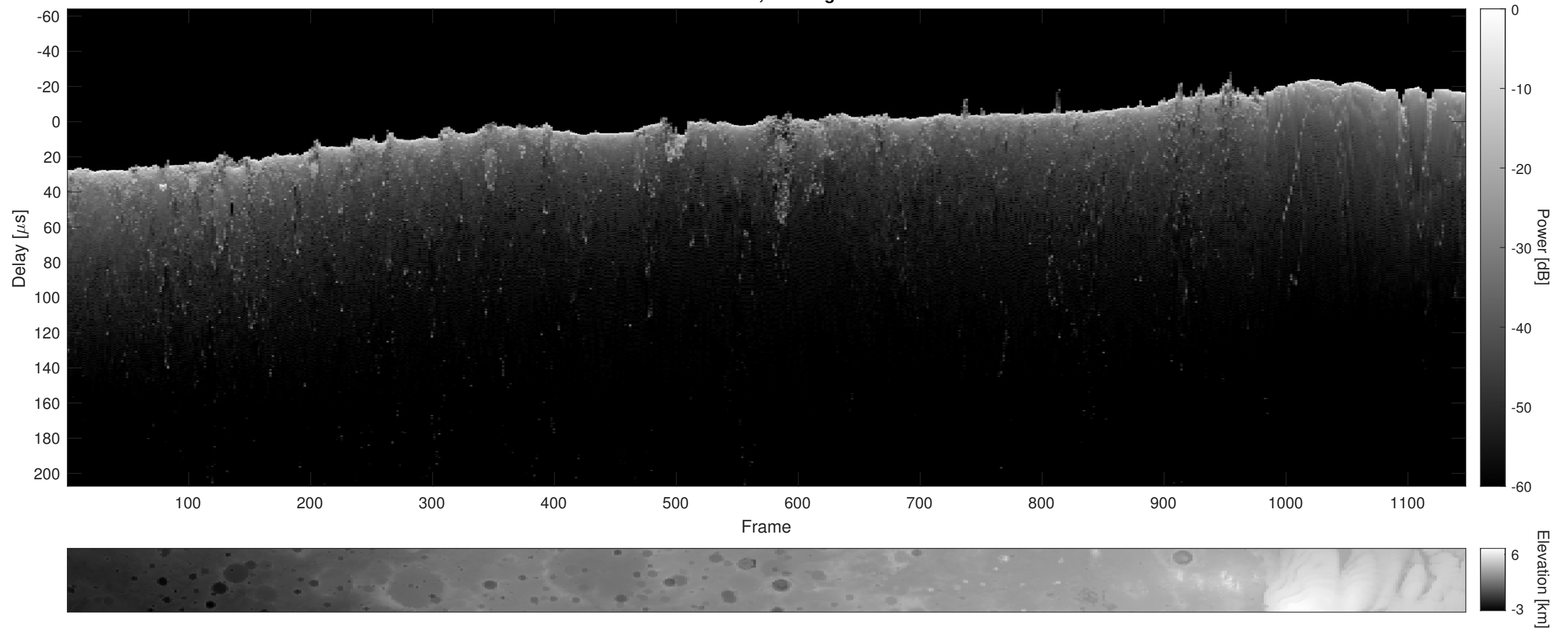
Orbit 13168, Cluttergram
