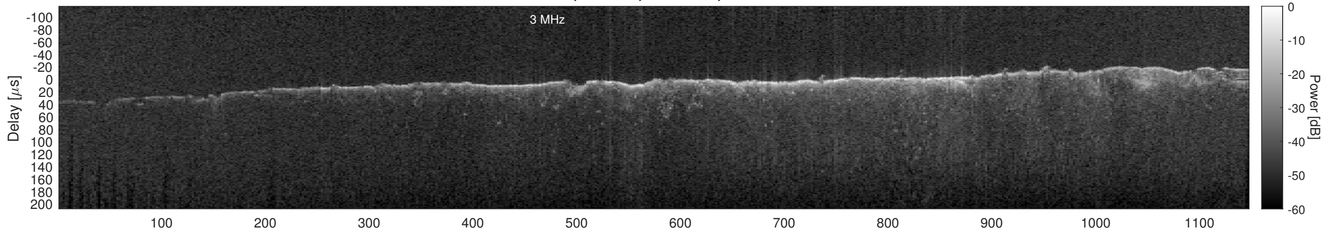
Orbit 13168, Window, Channel 2, Chapman
