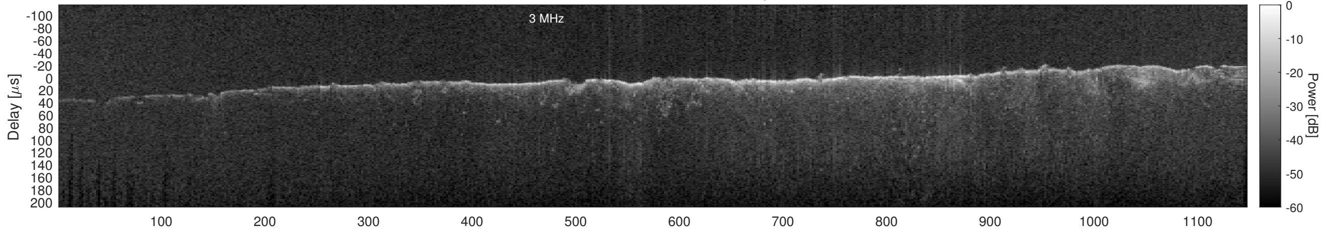
Orbit 13168, Window, Channel 2, Optimized
