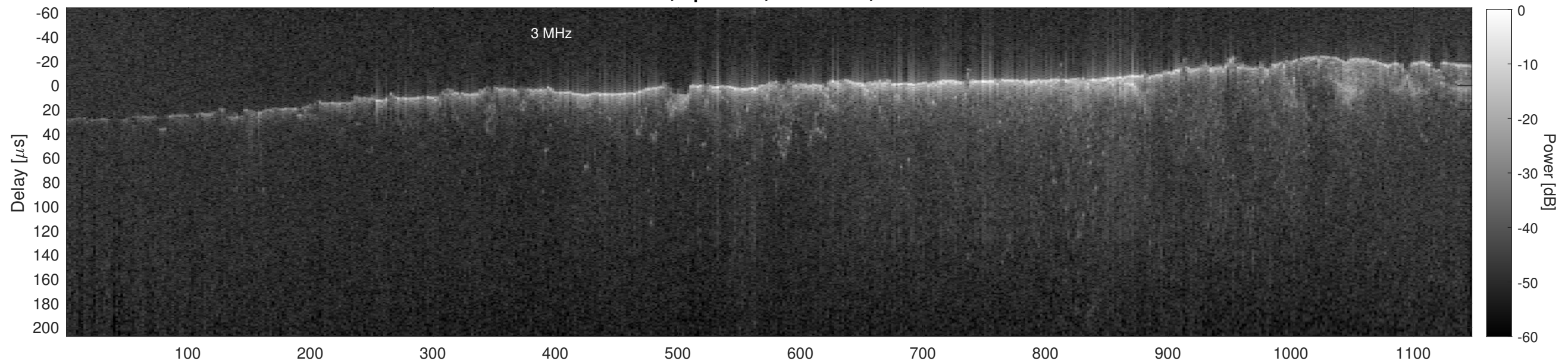
Orbit 13168, Cluttergram
