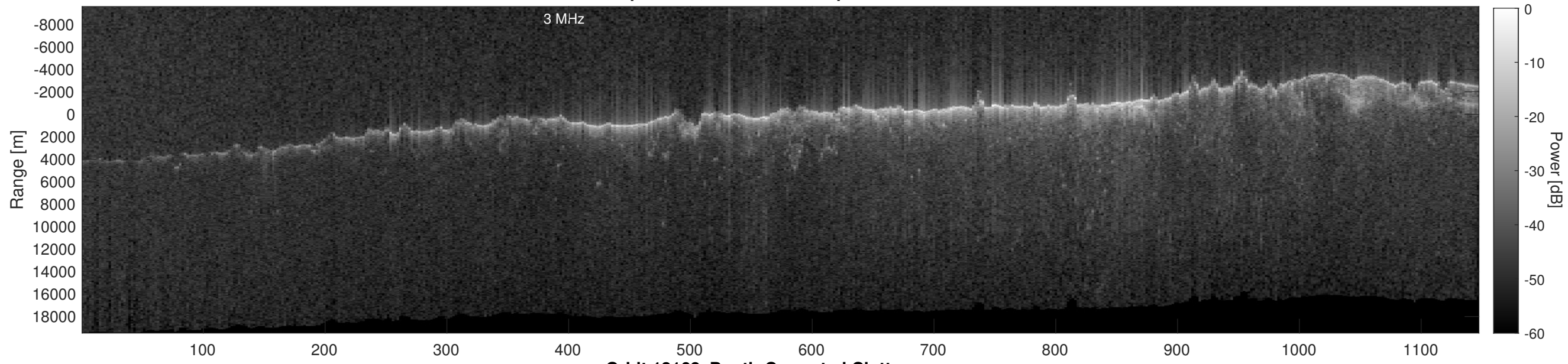
Orbit 13168, Depth-Corrected Cluttergram
