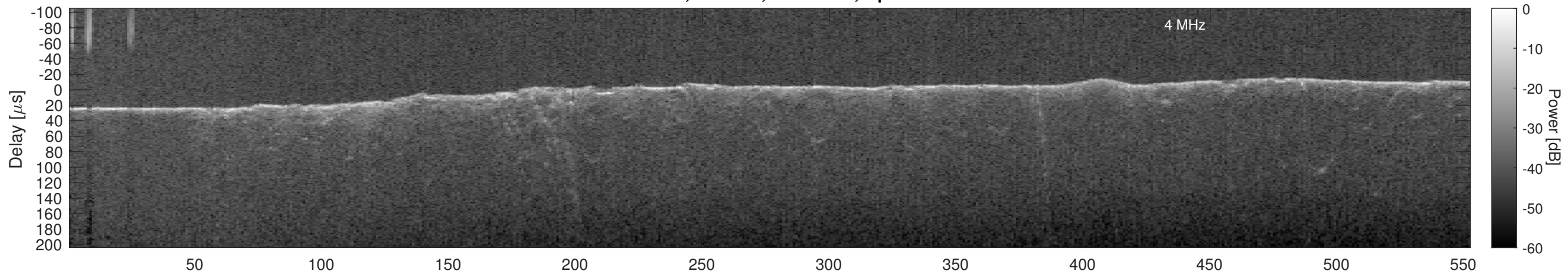
Orbit 13170, Cluttergram
