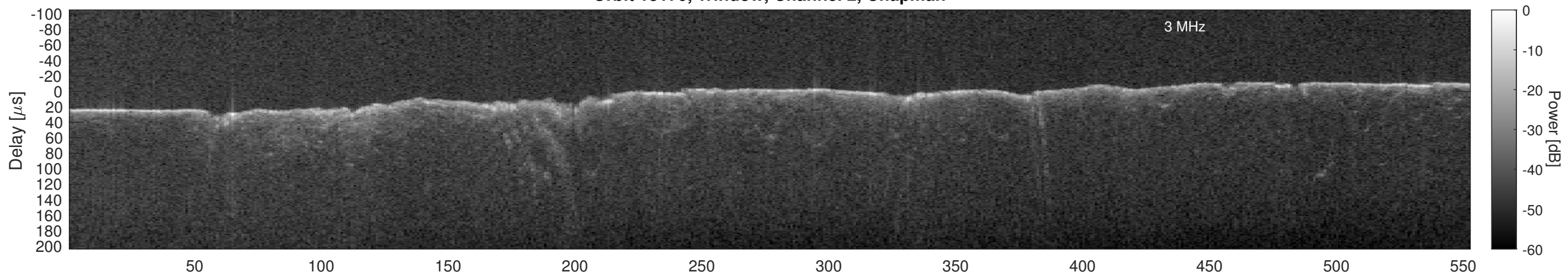
Orbit 13170, Window, Channel 2, Optimized
