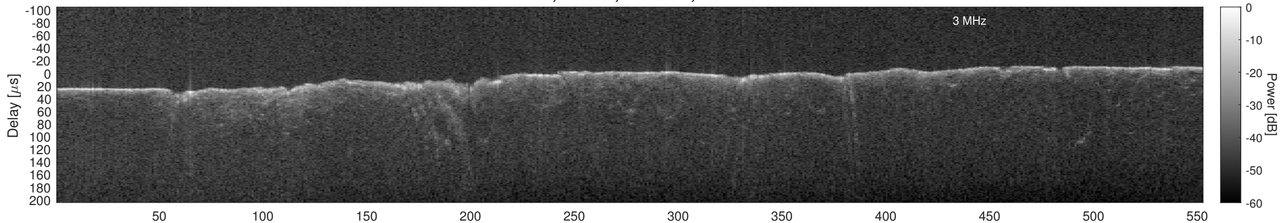
Orbit 13170, Window, Channel 2, Chapman
