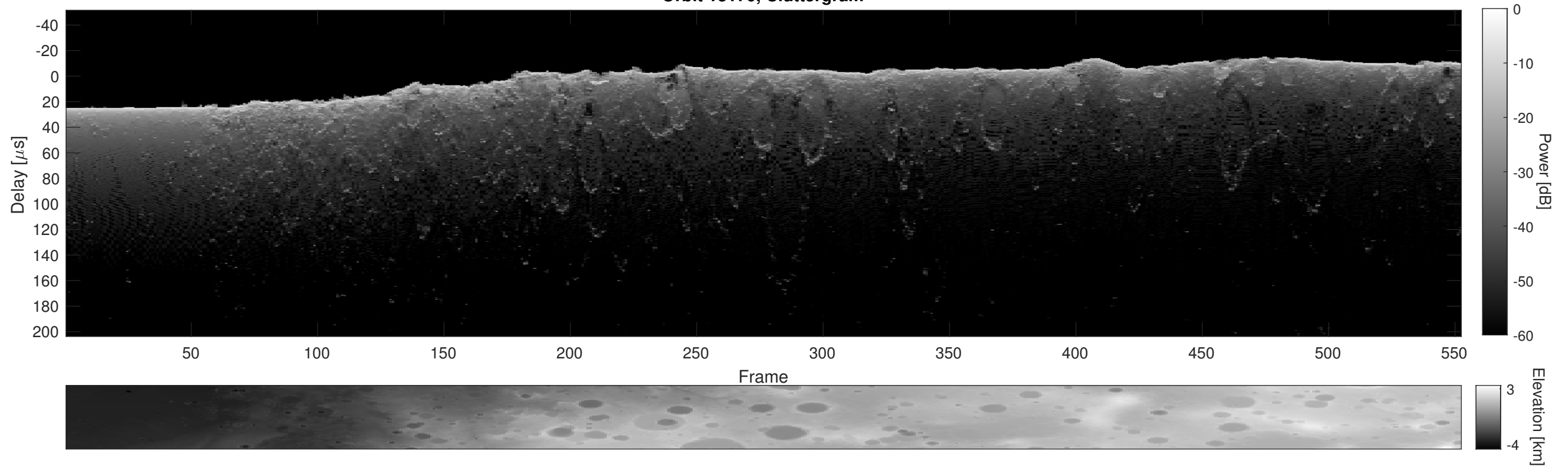
Orbit 13170, Cluttergram
