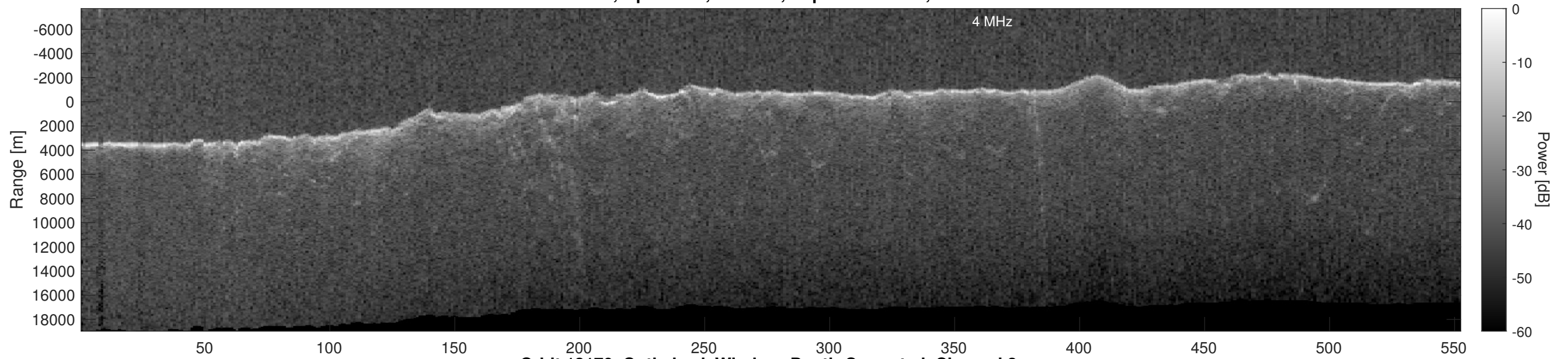
Orbit 13170, Optimized, Window, Depth-Corrected, Channel 2
