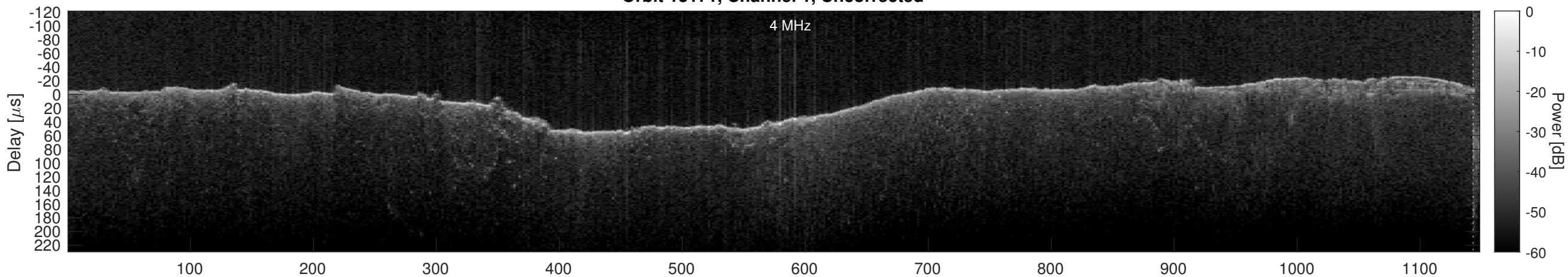
Orbit 13171, Window, Channel 1, Chapman
