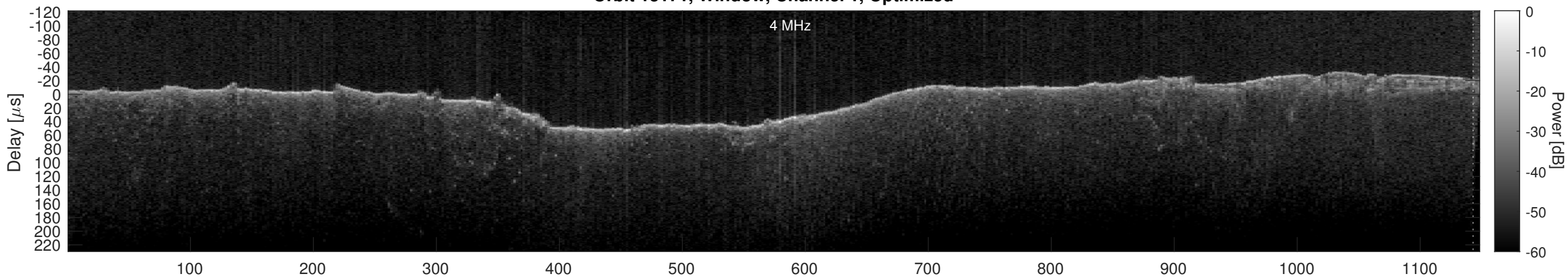
Orbit 13171, Cluttergram
