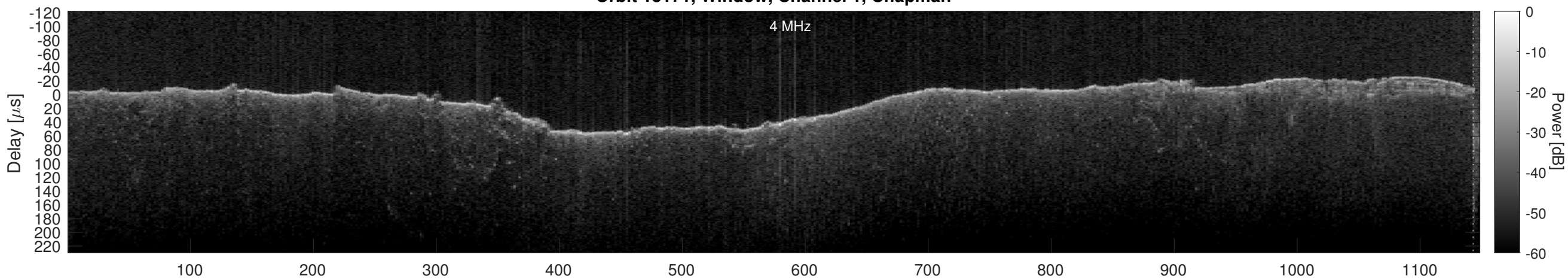
Orbit 13171, Window, Channel 1, Optimized
