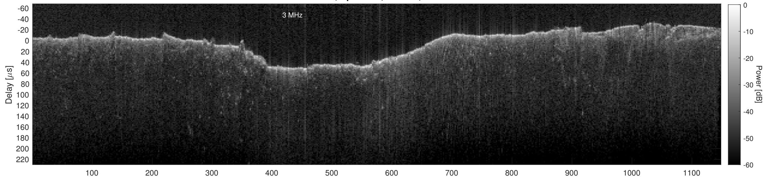
Orbit 13171, Cluttergram
