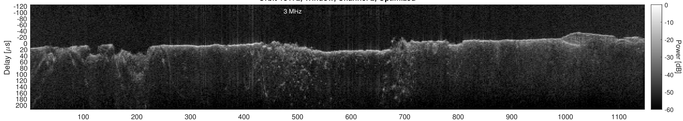
Orbit 13172, Cluttergram
