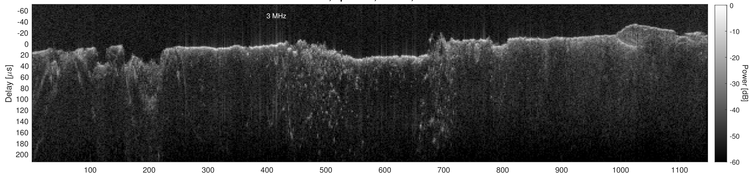
Orbit 13172, Cluttergram
