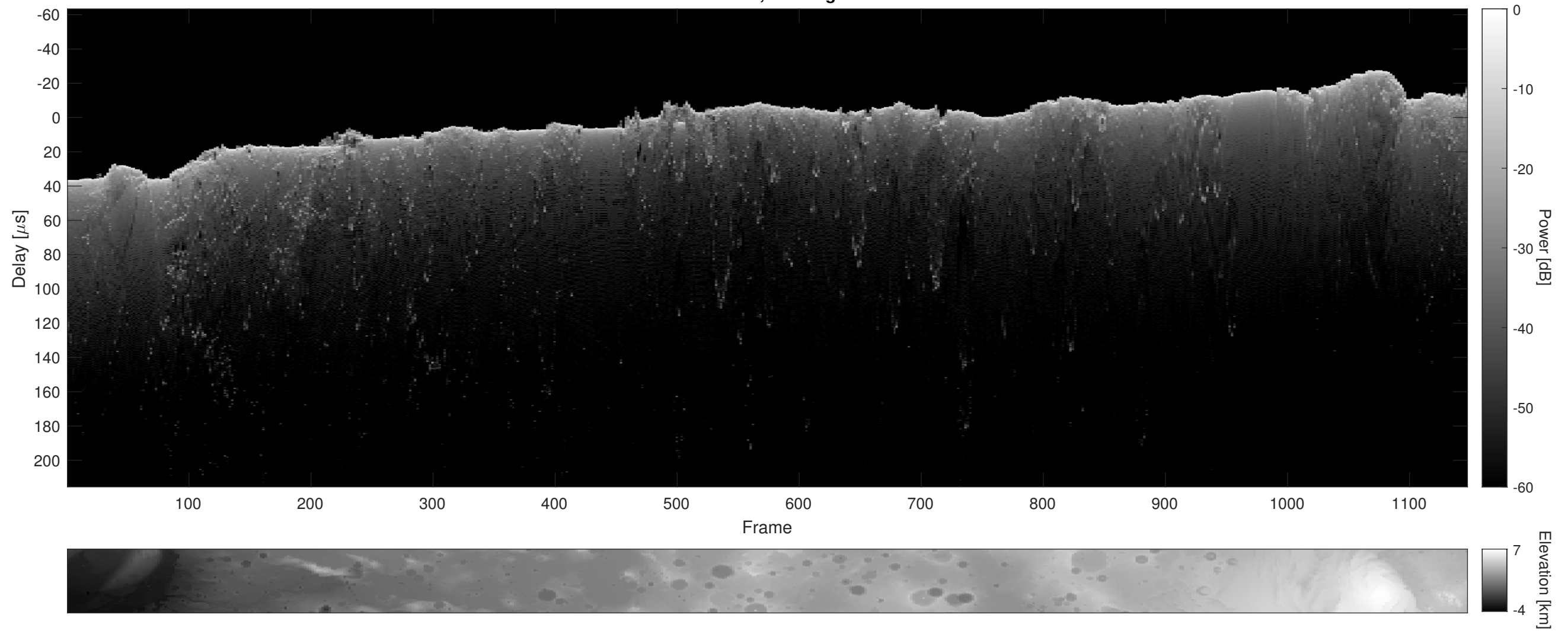
Orbit 13173, Cluttergram
