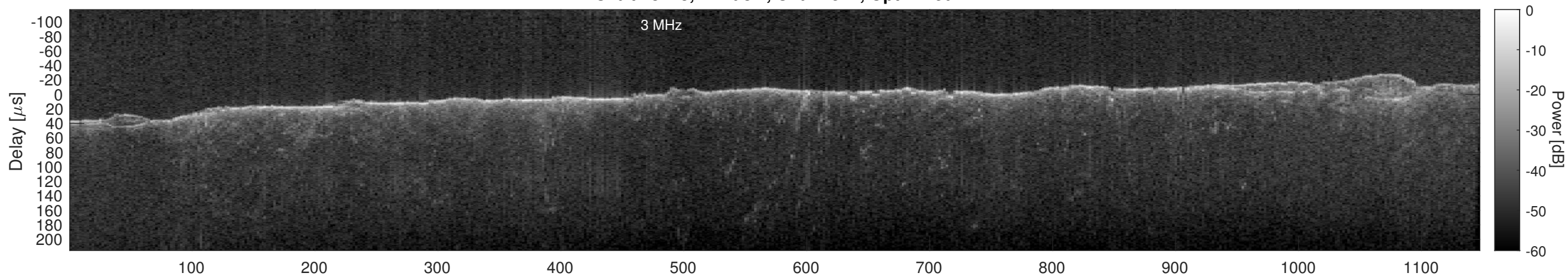
Orbit 13173, Cluttergram
