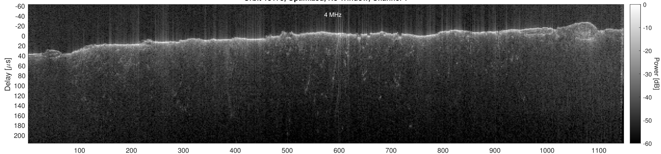
Orbit 13173, Optimized, No Window, Channel 2
