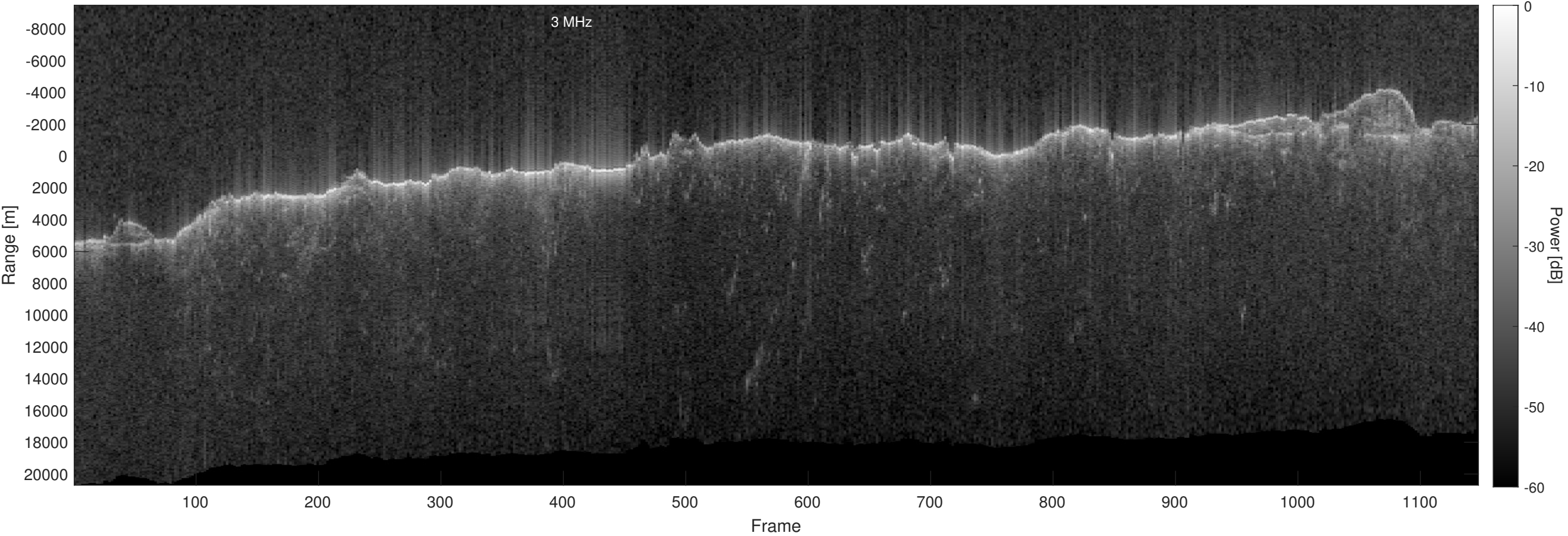
Orbit 13173, Optimized, No Window, Depth-Corrected, Channel 2
