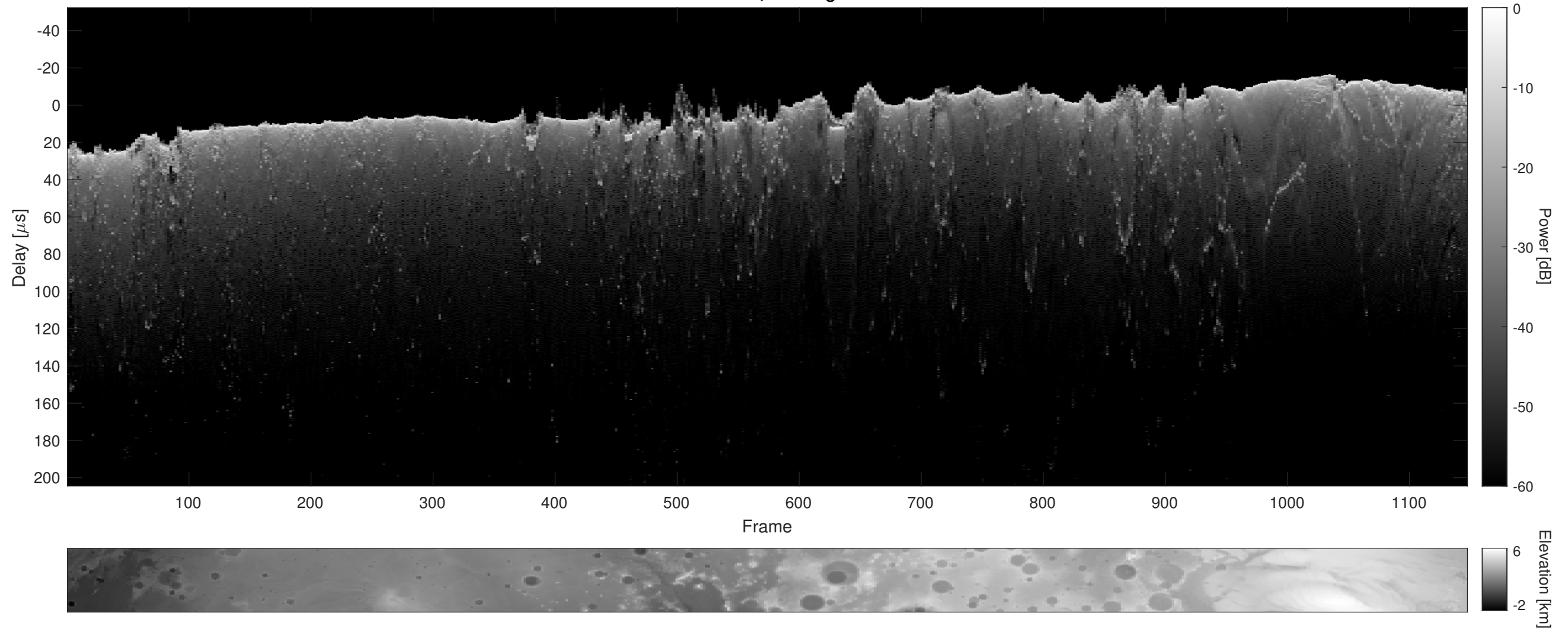
Orbit 13174, Cluttergram
