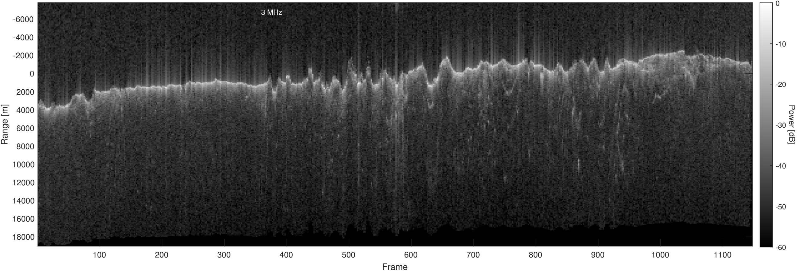
Orbit 13174, Optimized, No Window, Depth-Corrected, Channel 2
